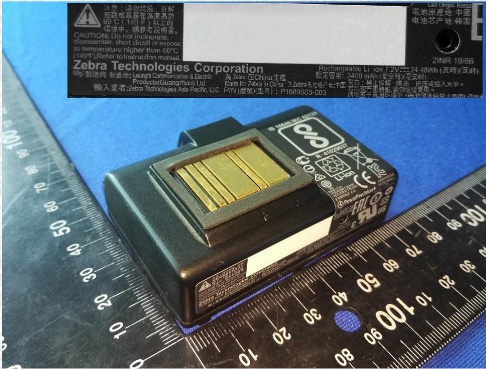
Battery (P1089503-003 7,2V 3400mAh 24,48Wh)
