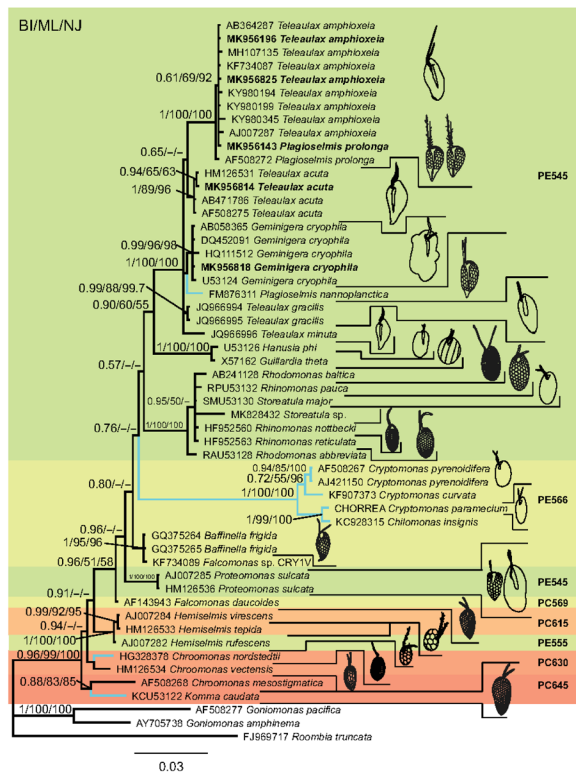
Fig. 2. Phylogeny of cryptophytes analyzed by Bayesian inference of 18S rDNA sequences. Numbers at nodes represent the posterior probability of Bayesian analysis/bootstraps values of maximum likelihood out of 1000 replicates/bootstraps values of neighbor-joining out of 10,000 replicates. Not resolved branches and branches with support values below 50% are marked with a minus sign (-). The scale bar corresponds to three substitutions per 100 nucleotide positions. Colors correspond to absorption maxima (i.e., PE545 = green). Branches for freshwater species are blue, marine and brackish species are black. Newly sequenced strains are in bold. Drawings of cells are not to scale.
