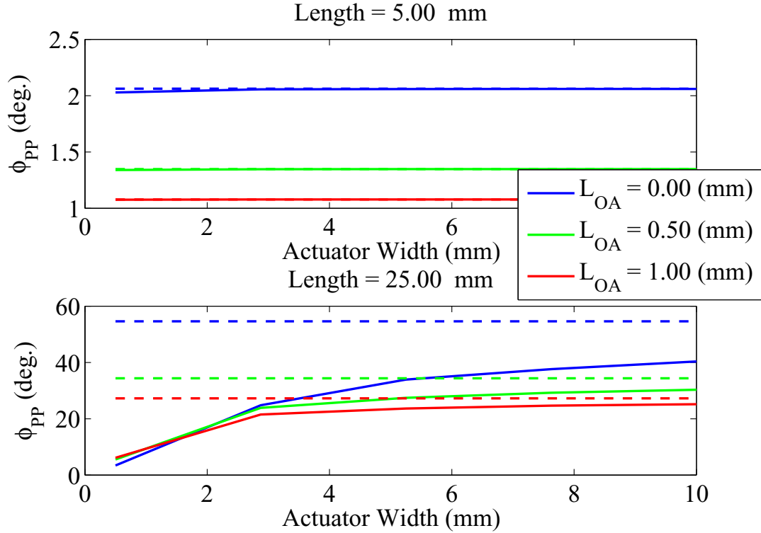
Figure B.1.5. \phi_{PP} versus actuator width, L_{OA} with applied voltage of \pm 150 V , \phi_0 = 45^\circ : (solid) calculated \phi by solved bimorph displacement, (dashed) \phi calculated by bimorph free displacement
