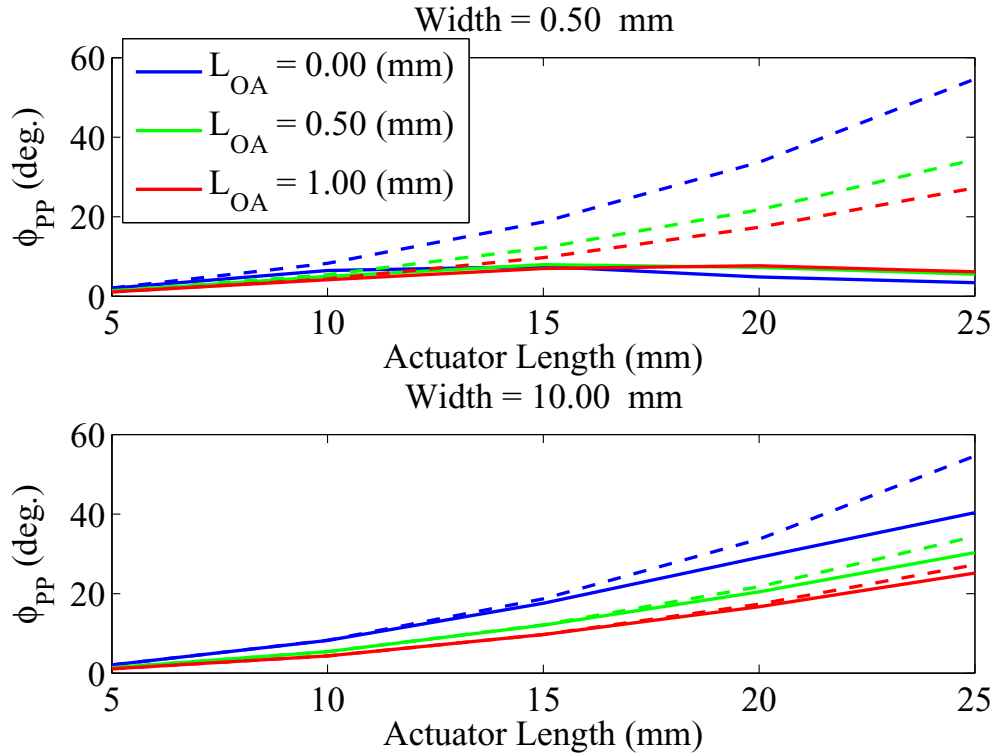
Figure B.1.4. \phi_{PP} versus actuator length, L_{OA} with applied voltage of \pm 150 V , \phi_0 = 45^\circ : (solid) calculated \phi by solved bimorph displacement, (dashed) \phi calculated by bimorph free displacement
