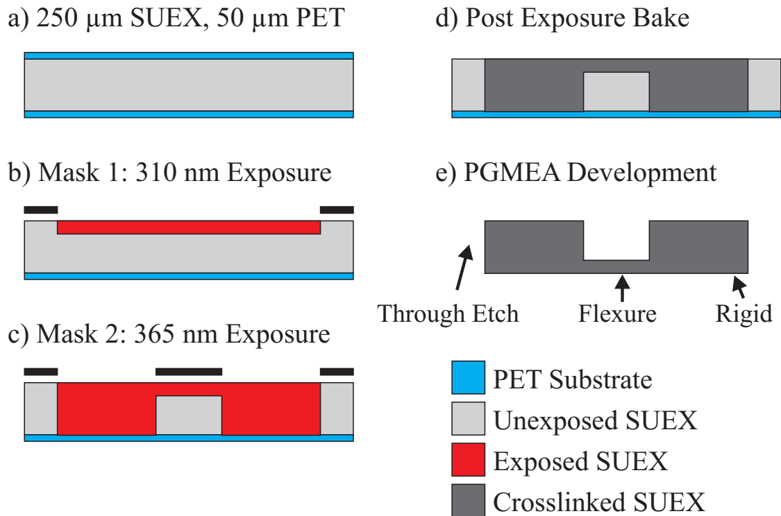
Figure 3.2.3. Fabrication of SUEX structure: (a) initial SUEX substrate between two 50\ \mu\text{m} PET layers, (b) 310\ \text{nm} exposure dose of 500\ \text{mJ}/\text{cm}^2 for 25\ \mu\text{m} flexure layer, (c) 365\ \text{nm} exposure dose of 1350\ \text{mJ}/\text{cm}^2 for 250\ \mu\text{m} rigid layer, (d) post exposure bake ( 65^\circ for 30 min) to activate cross linking in SUEX, (e) development in PGMEA for 1 hr with light agitation releases structures
