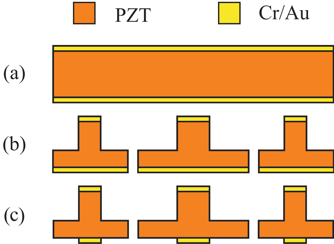
Figure 2.2.1. NAV T-beam fuselage fabrication process: (a) 25.4 mm \times 25.4 mm \times 1 mm finely polished, Cr/Au electroded PZT-5H chip (b) machining of PZT using high precision dicing saw (c) patterning of bottom electrode
