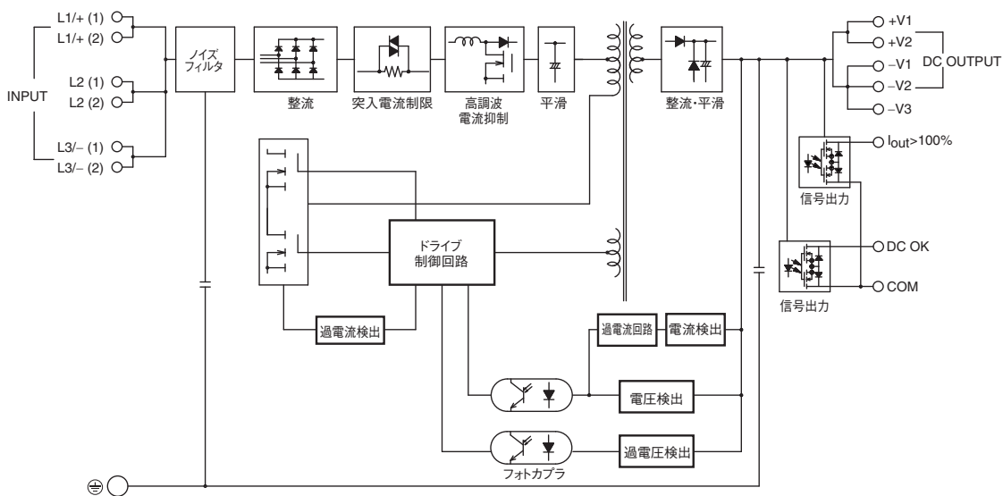
形S8VK-WA24024 (240W)
