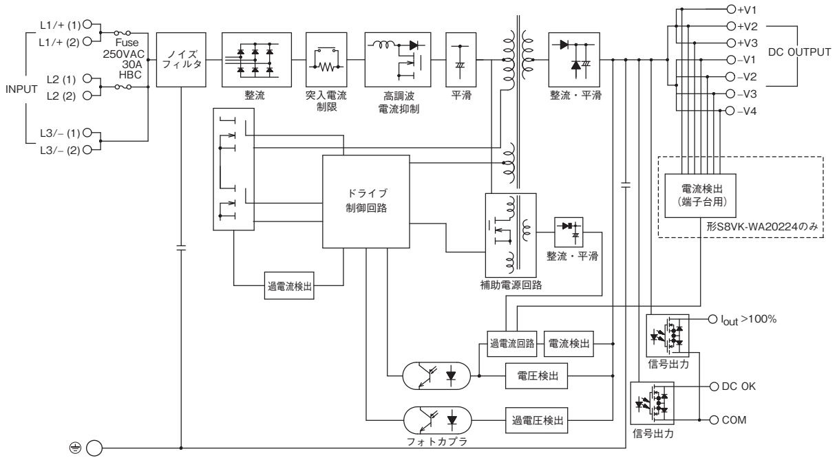
形S8VK-WA202□□ (2000W)
