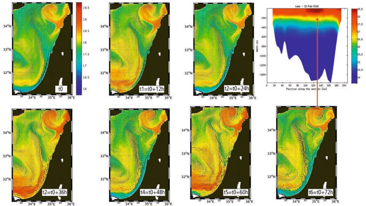
Figure 1a: Example: Eastern Mediterranean Sea. Prediction points for the temperature parameter at the ocean surface over 72 hours. The northern boundary of the model area is shown as an example of a vertical section, from the island of Cyprus to Syria and from the sea surface to the sea bed. The distinctive vortex of warm water (red arrow) is found both in the vertical section and the horizontal representation.
