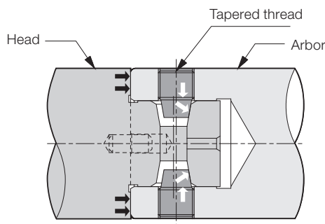
Strong rigid connection between Boring Head and Arbor.
