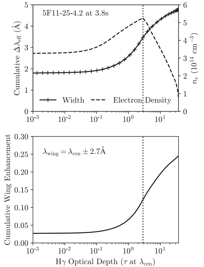
Figure 7. Top: the curve-of-growth of the effective width of H\gamma through the chromospheric condensation at t = 3.8 s in the 5F11 model. The physical depth range in this figure is \Delta z \approx 30 km. At larger optical depths than at the maximum of n_e (vertical dotted line), the widths of the line increase further until reaching values near 4.9 Å in the emergent intensity spectrum. Bottom: the cumulative of the contribution function at \lambda_{\text{cen}} \pm 2.7 Å relative to the cumulative of the contribution function at \lambda_{\text{cen}} . This closely follows the cumulative variation in effective width in the top panel.
