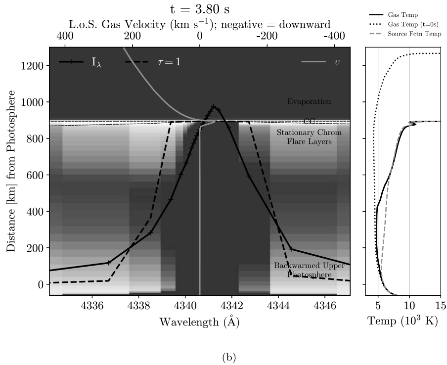
Figure 6. Contribution function to the emergent intensity ( \mu = 0.95 ) of H\gamma at (a) t = 0 s and at (b) t = 3.8 s in the 5F11-25-4.2 model. The shading ranges logarithmically ( \log_{10} ) from 0.001 (red/brown) to 1 (white/yellow) in units of \text{erg s}^{-1} \text{cm}^{-2} \text{sr}^{-1} \text{\AA}^{-1} \text{cm}^{-1} in both panels. The cumulative contribution-function surfaces are shown for 10% (upper dotted curve) and 90% (lower dotted curve) of the emergent intensity at t = 3.8 s, calculated using only layers above 400 km. The line-of-sight (LOS) gas velocity v is defined as \mu v_z where \mu is related to the viewing angle \cos \theta , and v_z is the gas velocity along the loop. The side panels in each figure on the right show the atmospheric temperature and the bound-bound source function equivalent temperature. The departures from LTE over 3 km at the top of the condensation (at the temperature increase from 10,000 to 25,000 K) are significant but are not apparent on this scale.
