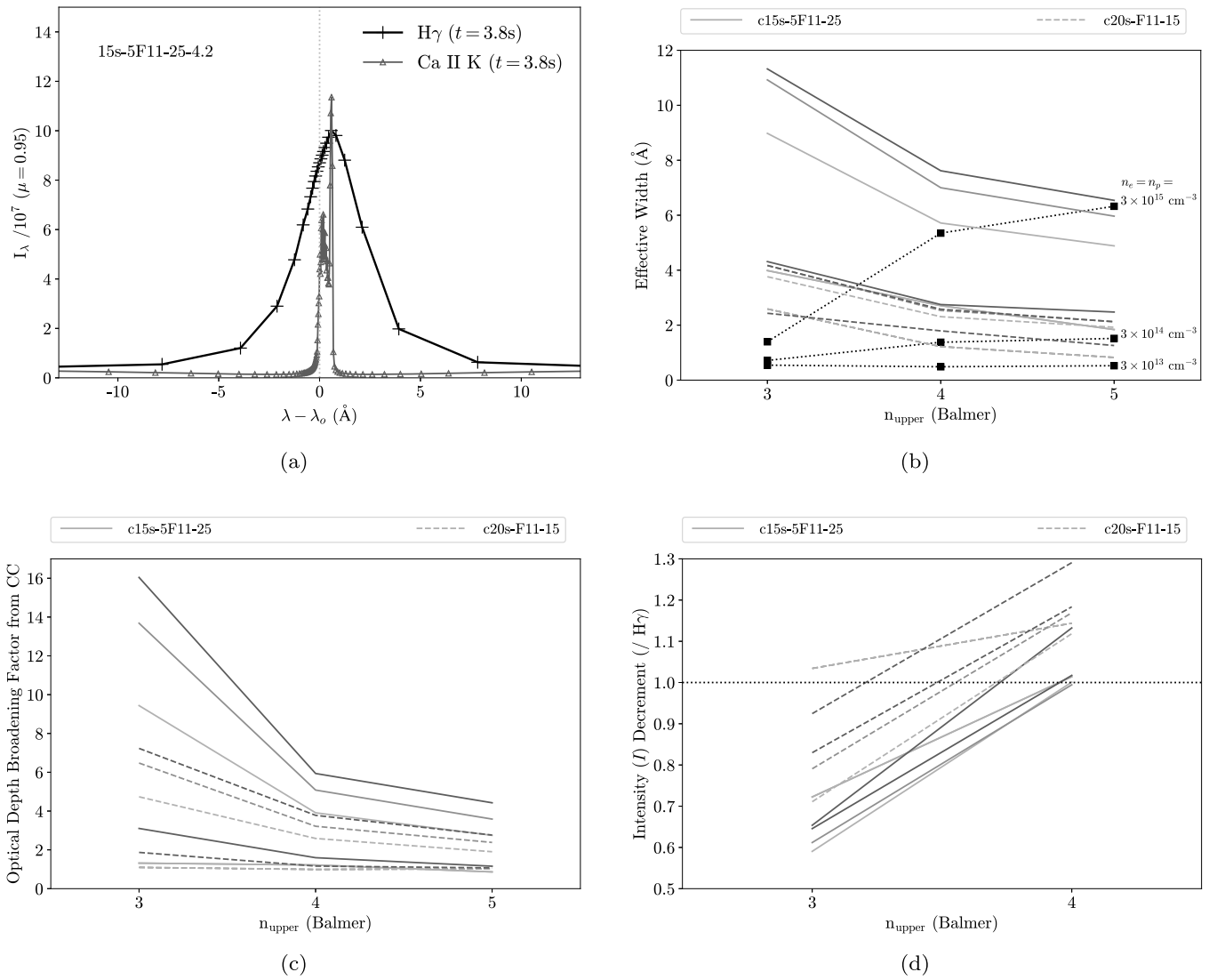
Figure 8. Comparisons of several optical emission lines in the flare models. (a) Large differences in the broadening of H\gamma and Ca II K in the 5F11–25–4.2 model agree qualitatively with the observed phenomena in solar and stellar flares (e.g., Neidig 1983). (b) Evolution of the effective widths of the H\gamma , H\beta , and H\alpha lines in the 5F11–25–4.2 and F11–15–5 models. The effective width trends of the TB09+HM88 profiles without optical-depth effects (black dashed lines) for several representative ambient electron densities increase up the series, as expected. (c) Optical-depth broadening factors through the chromospheric condensation (CC) increase from H\gamma to H\alpha . The effective widths in the broadening factors were calculated from the cumulative contribution function at the deepest height of the condensation at each time step. Note that the optical-depth broadening factor of H\gamma at t = 1 s in the 5F11 model is slightly less than 1, which is due to a low but nonnegligible ( \approx 0.1 ) optical depth in the condensation and velocity gradients that lead to broadening in the \tau = 0 calculation. (d) The Balmer decrement with respect to H\gamma . In panels (b), (c), and (d), the color coding according to time is the same as in Figures 5(a)–(b).
