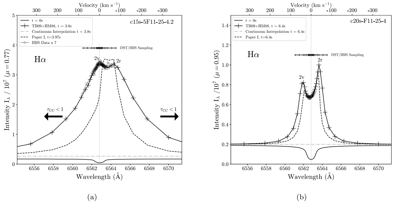
Figure 3. Model H\alpha flare spectra using the TB09+HM88 profiles in RADYN. These are improvements on recent works (dashed lines), which used the profiles corresponding to the broadening implementation of spectrum (4) in Figure 1(a). These two snapshots were chosen as the most similar in time to the snapshots that were analyzed in Figure 8 of Paper I (panel (a) here) and in Figure 7 in Kuridze et al. (2015; panel (b) here). In this figure, the same viewing angles ( \mu ) are presented as in these two previous works. The flare continuum emergent intensity is interpolated across the line to demonstrate that in the higher beam flux model, the wings of the H\alpha line extend beyond this wavelength range ( \Delta\lambda = 17.15 \text{ \AA} , chosen as a representative wavelength range of a DKIST/ViSP window). The arrows in the left panel indicate the wavelengths at which the chromospheric condensation becomes optically thin over the TB09+HM88 spectrum (see text).
