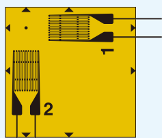
ZFCA-1-350-11 (x 3)
