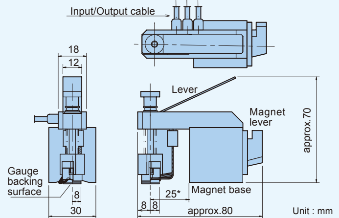
FGMH-3A (0°/45°/90° Three-axis)
