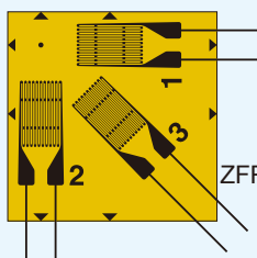
ZFCA-1-350-11 (x 3)
