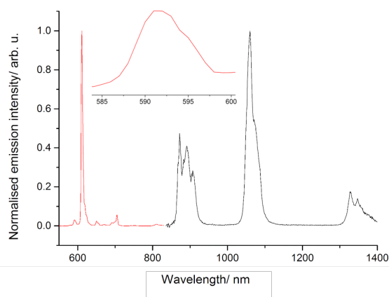
Figure 3 Normalised emission plot for \{[\text{Eu}(\text{Rb})(\text{mtbm})_4]_2\}_n (red trace) and \{[\text{Nd}(\text{Rb})(\text{mtbm})_4]_2\}_n (black trace) in the solid state, with excitation wavelength at 350nm. Inset: highlight of the splitting of the magnetic dipole transition for the \text{Eu}^{3+} complex.
