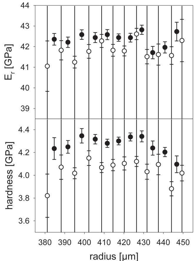
FIG. 11. Averaged values of reduced modulus (upper part) and hardness (lower part) of the indents within each silica layer as a function of the distance from the center of a M. chuni spicule (radius). Indents touching the organic interlayer (open symbols) and away from the interlayer (full symbols) are analyzed separately. The gray vertical lines show the positions of the organic interlayers.
