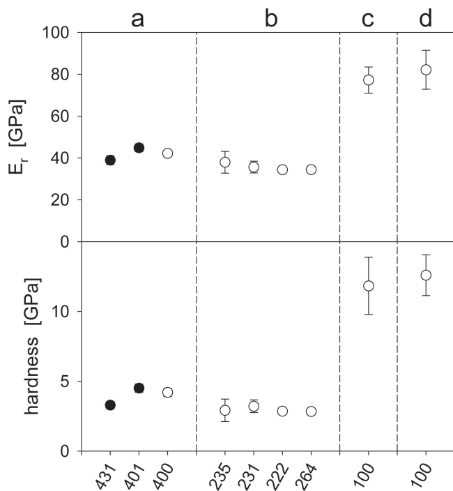
FIG. 14. Summary of the nanoindentation experiments for (a) spicules of M. chuni , (b) spicules of E. aspergillum , and technical quartz glass with (c) low and (d) high \text{OH}^- content. Average reduced modulus ( E_r ) and hardness are plotted with error bars representing standard deviations. The numbers on the abscissa correspond to the quantity of indents used for each evaluation. Closed symbols indicate line scans and open symbols area scans.
