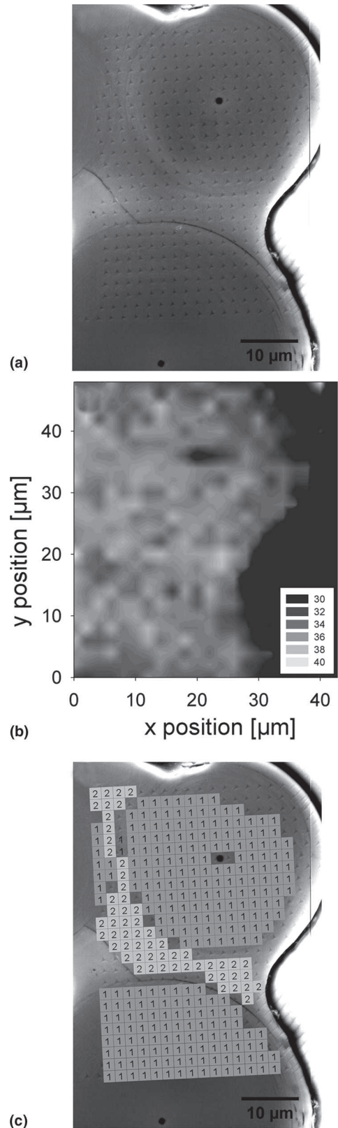
FIG. 13. Micromechanical testing of bundles of spicules from E. aspergillum : (a) array of indents visualized by backscattered electron imaging, (b) reduced modulus map from nanoindentation, and (c) assignment of the indents to different regions (1 = spicule, 2 = cement).
