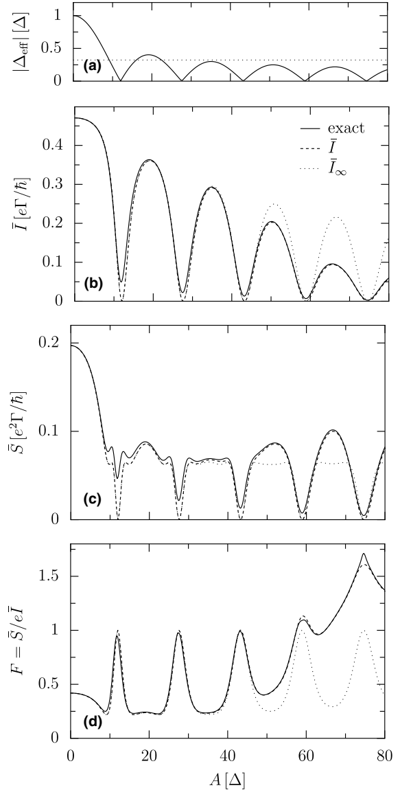
Fig. 4. (a) Effective hopping matrix element |\Delta_{\text{eff}}| , (b) time-averaged current \bar{I} , (c) zero-frequency noise \bar{S} , and (d) Fano factor F = \bar{S}/e\bar{I} as a function of the driving amplitude A . Shown are the numerically exact results (solid lines), the approximate results (31) and (32) for finite voltage (dashed lines), and the infinite voltage results (20) and (21) with A replaced by \Delta_{\text{eff}} (dotted lines). The coupling strength is \Gamma = 0.5A , the driving frequency is \Omega = 5A/\hbar , and the voltage reads V = 48A/e . The dotted line in (a) marks the value \sqrt{5/12}\Gamma for which the Fano factor assumes its minimum.
