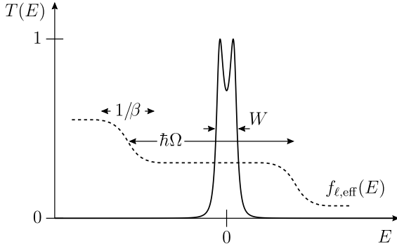
Fig. 3. Typical energy dependence of transmission T(E) (solid line) and effective distribution function f_{l,\text{eff}}(E) (dashed line) which allows to replace the distribution function by (30) in the expressions for current and noise.
