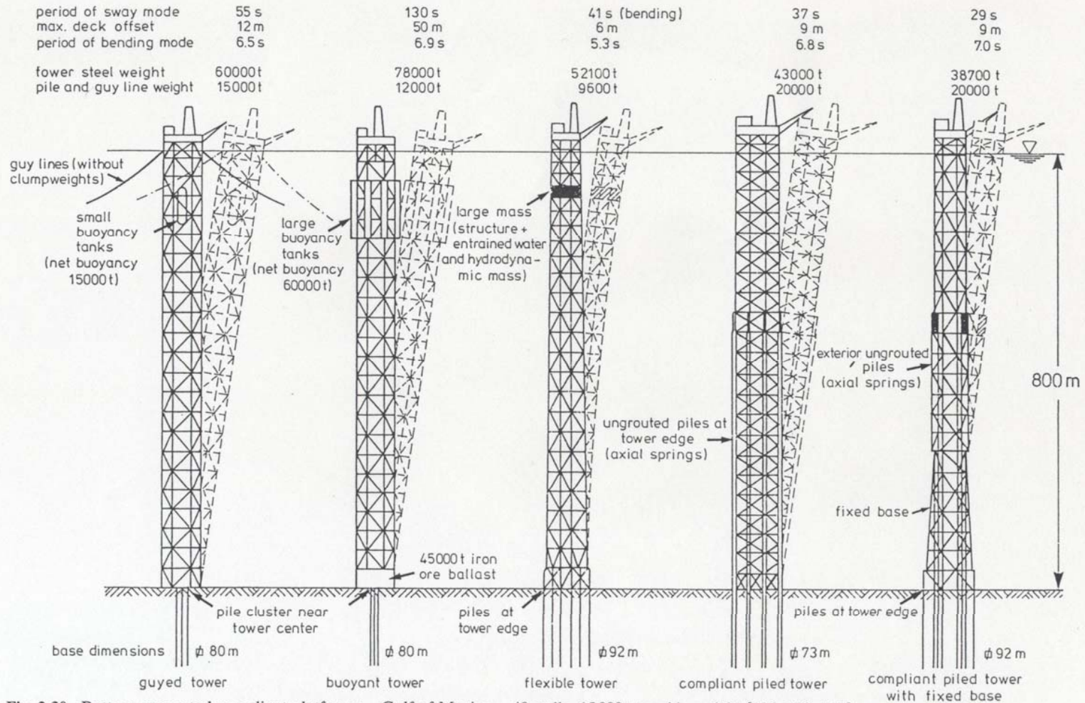
Fig. 2.30. Bottom-supported compliant platforms – Gulf of Mexico – 48 wells, 15 000 t topside weight [136, 139, 141].
